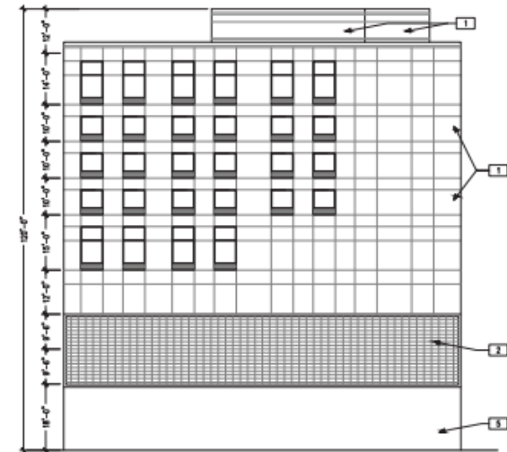
SOUTH ELEVATION SCALE: 1" = 20'-0"
