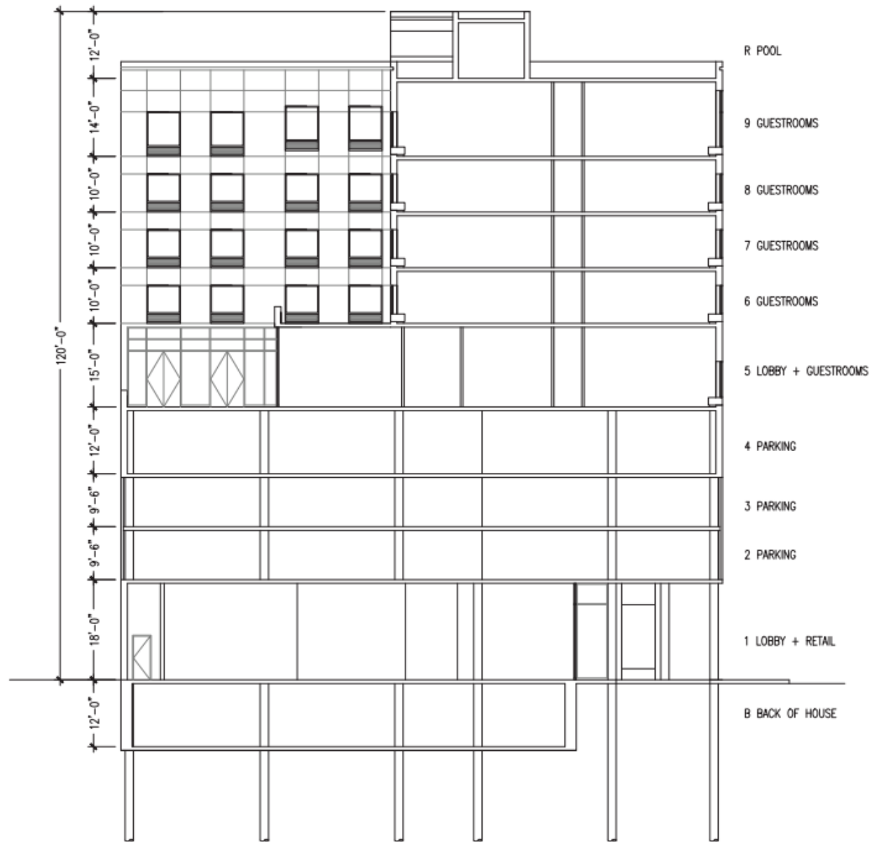
SECTION SCALE: 3/32" = 1'-0"
